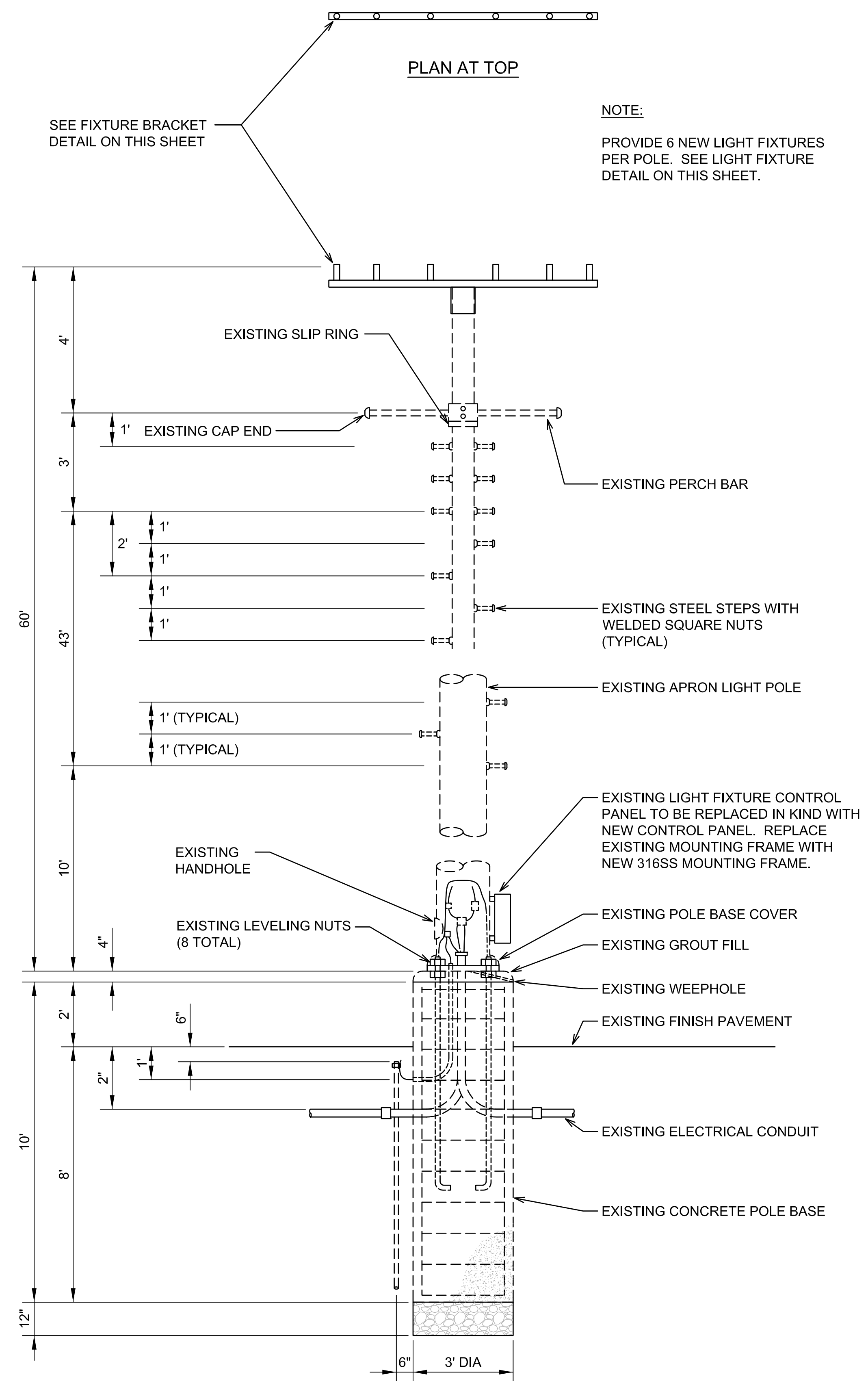
EXISTING ELEVATION
