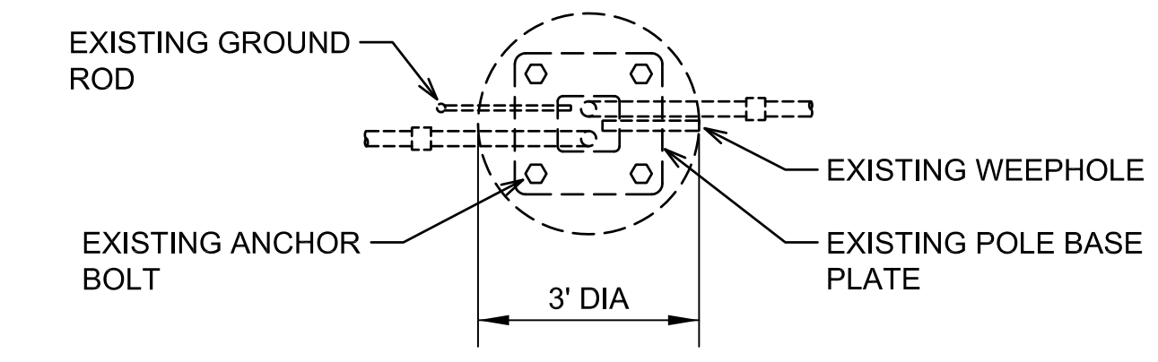
PLAN AT EXISTING POLE BASE
